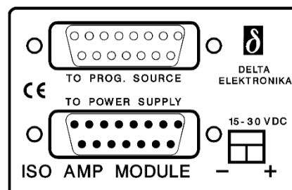
fig 4 - 1 Front panel connections.
