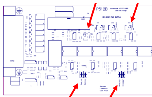
fig 5 - 1 Location of jumpers and trimmers on P512 revision B.
