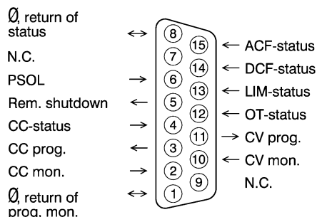
fig 4 - 3 To power supply.
