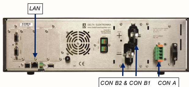
Figure 5.2: Connections on the rear side
