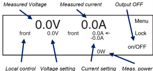
Figure 5.3: Actual output values and settings
